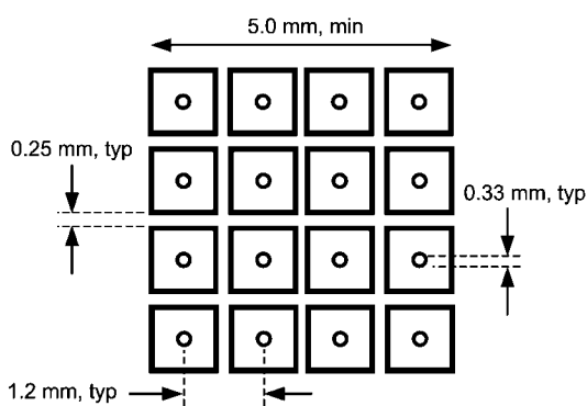
FIGURE 18. Recommended Package Land Pattern
