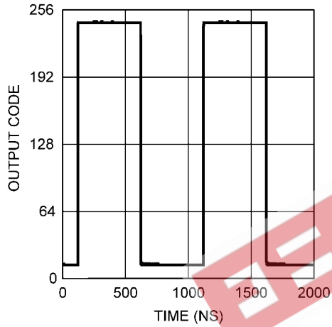
STEP RESPONSE
