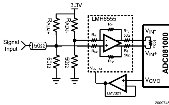
FIGURE 12. Example of Servoing the Analog Input with V_{CMO}
