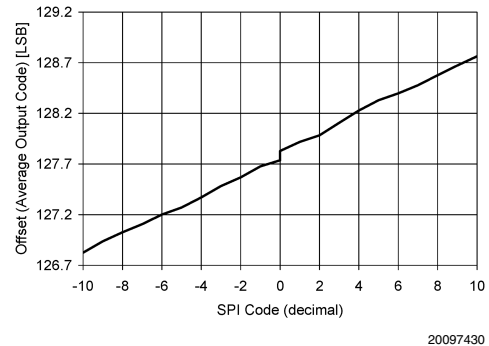
FIGURE 10. Extended Mode Offset Behavior
