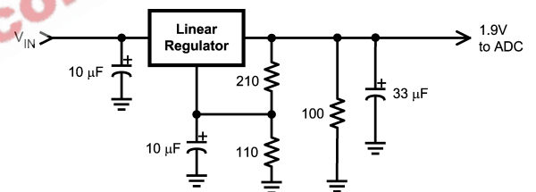
FIGURE 17. Non-Spiking Power Supply
