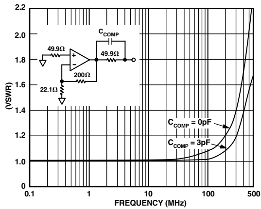
TPC 25. Output VSWR; G = +10
