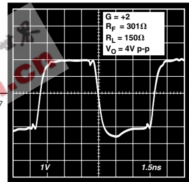
TPC 29. 4 V Transient Response; G = +2
