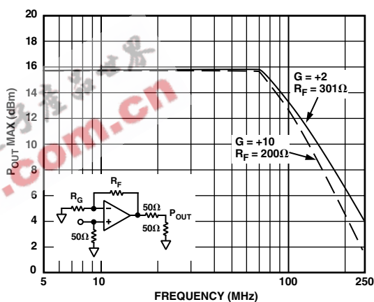
TPC 23. Maximum Output Power vs. Frequency
