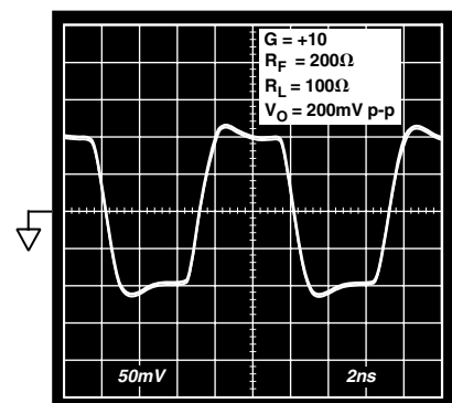
TPC 30. Small Signal Transient Response; G = +10
