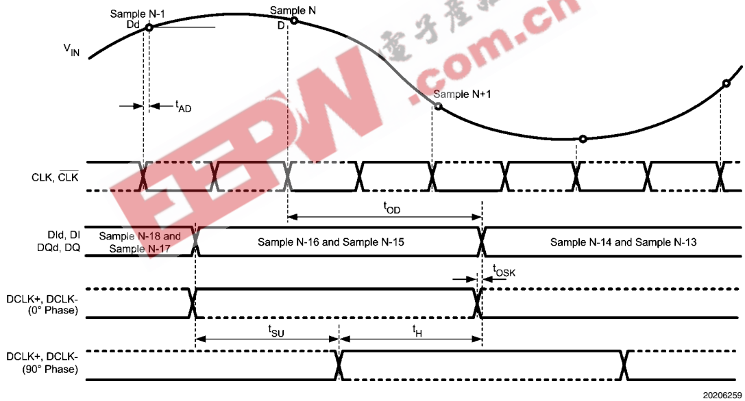
FIGURE 4. ADC08D1020 Timing — DDR Clocking in 1:2 Demultiplexed and Normal Mode
