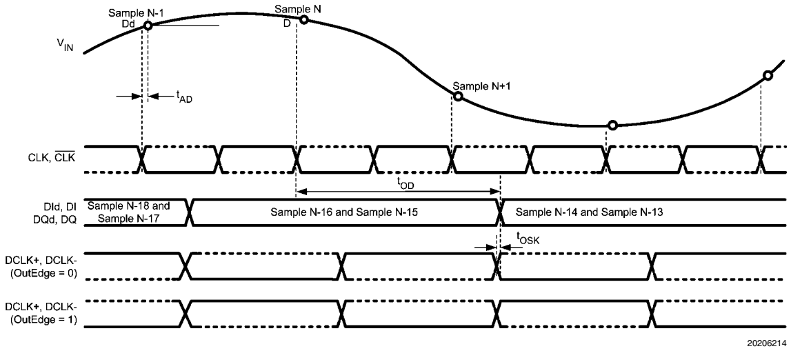
FIGURE 3. ADC08D1020 Timing — SDR Clocking in 1:2 Demultiplexed Mode
