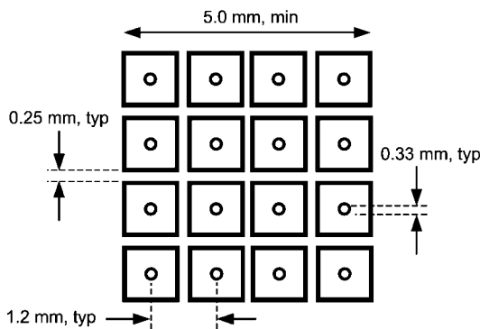
FIGURE 17. Recommended Package Land Pattern
