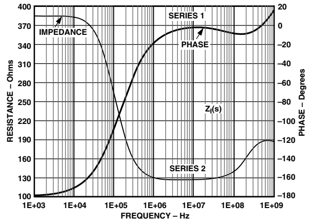
Figure 32. Open-Loop Inverting Input Impedance
