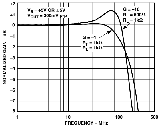
Figure 18. Frequency Response; G = -1, -10 ; V_S = +5\text{ V or } \pm 5\text{ V}
