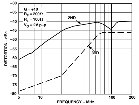
Figure 13. Distortion vs. Frequency; G = +10
