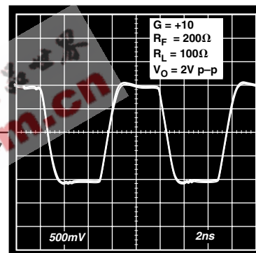
Figure 32. 2 V Transient Response; G = +10
