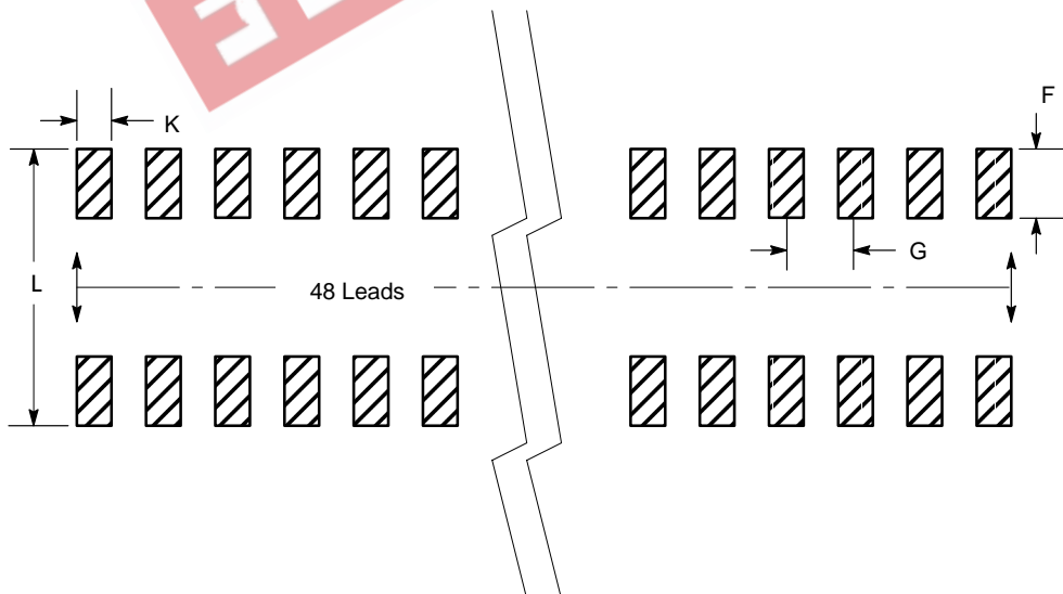
Figure 11. Package Footprint
