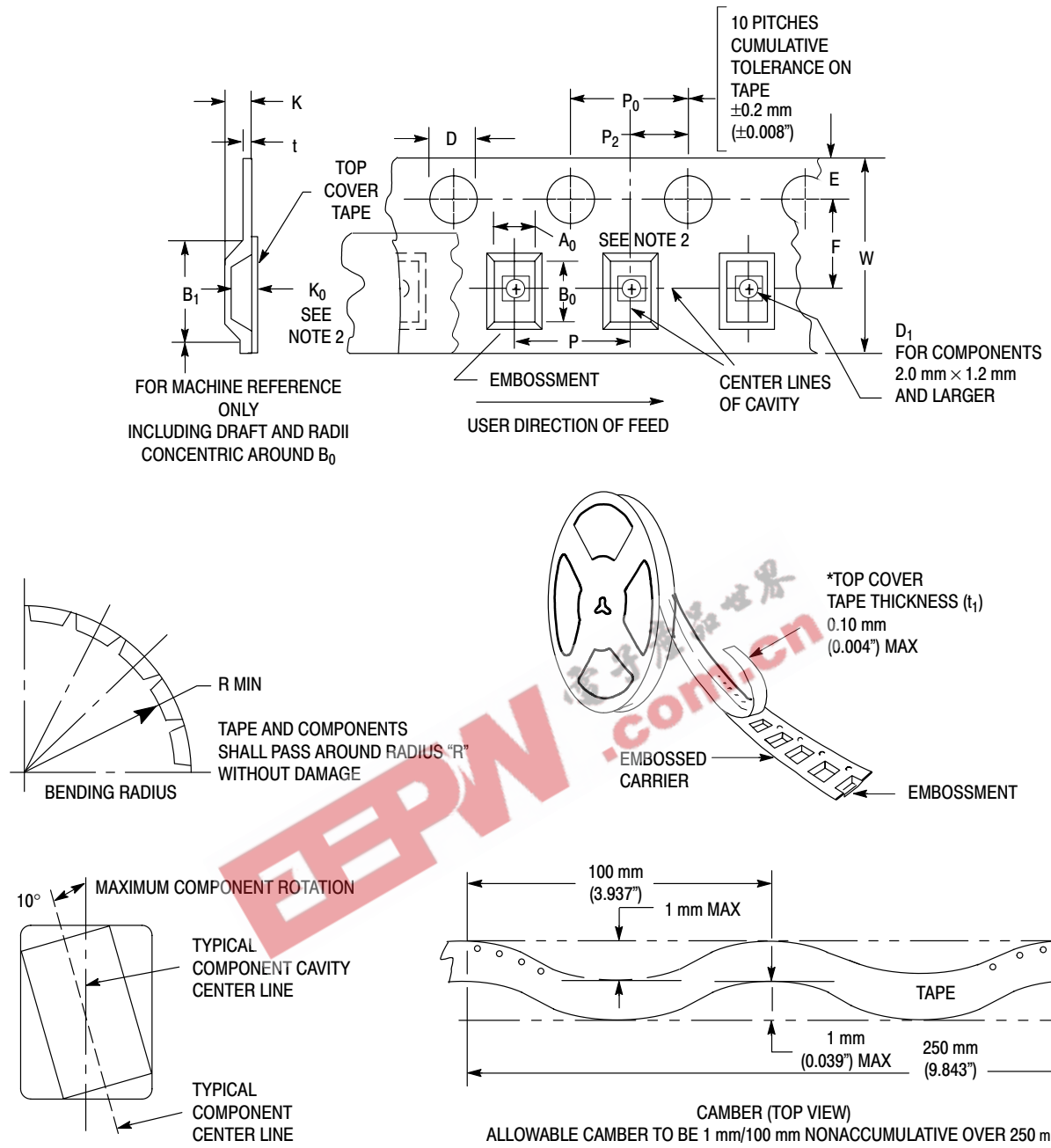
Figure 6. Carrier Tape Specifications
