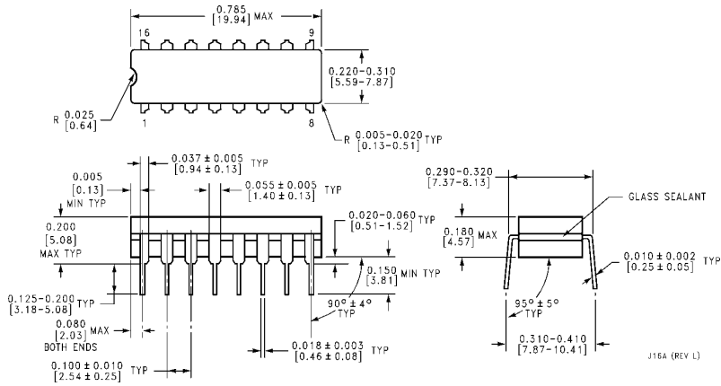
16-Lead Ceramic Dual-In-Line Package (J) Order Number 54LS352DMQB NS Package Number J16A
