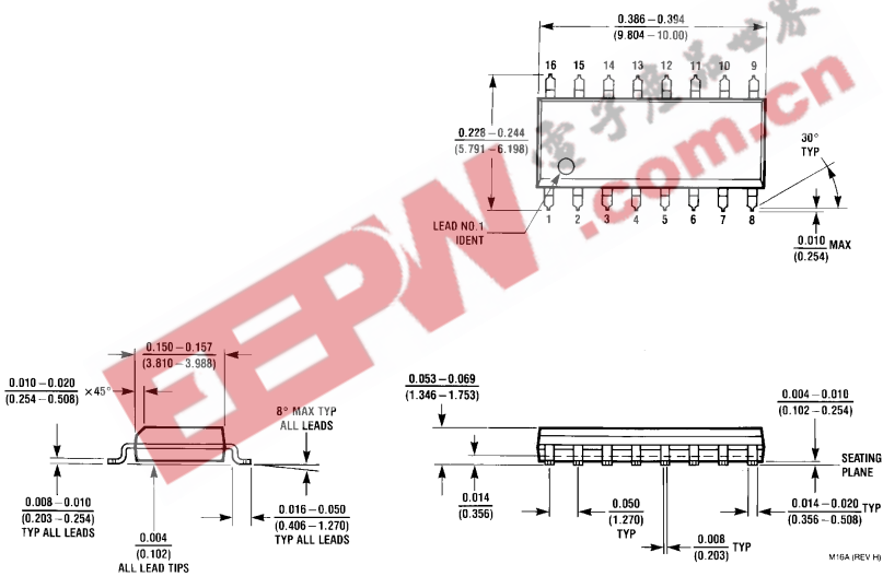
16-Lead Small Outline Molded Package (M) Order Number DM74LS352M NS Package Number M16A
