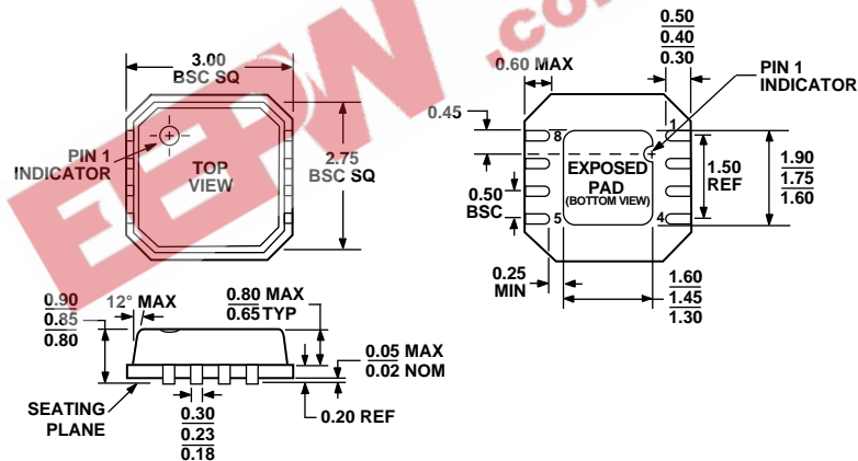
Figure 55. 8-Lead Lead Frame Chip Scale Package [LFCSP] 3 mm × 3 mm Body (CP-8-2) Dimensions shown in millimeters
