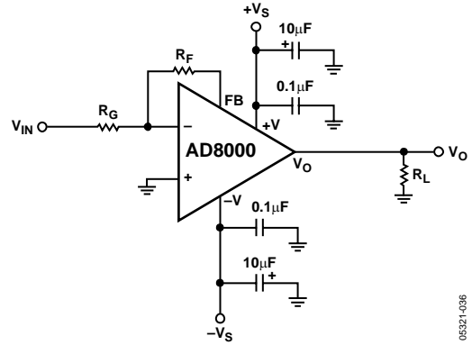
Figure 51. Inverting Configuration
