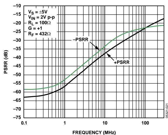
Figure 32. Power Supply Rejection Ratio (PSRR) vs. Frequency
