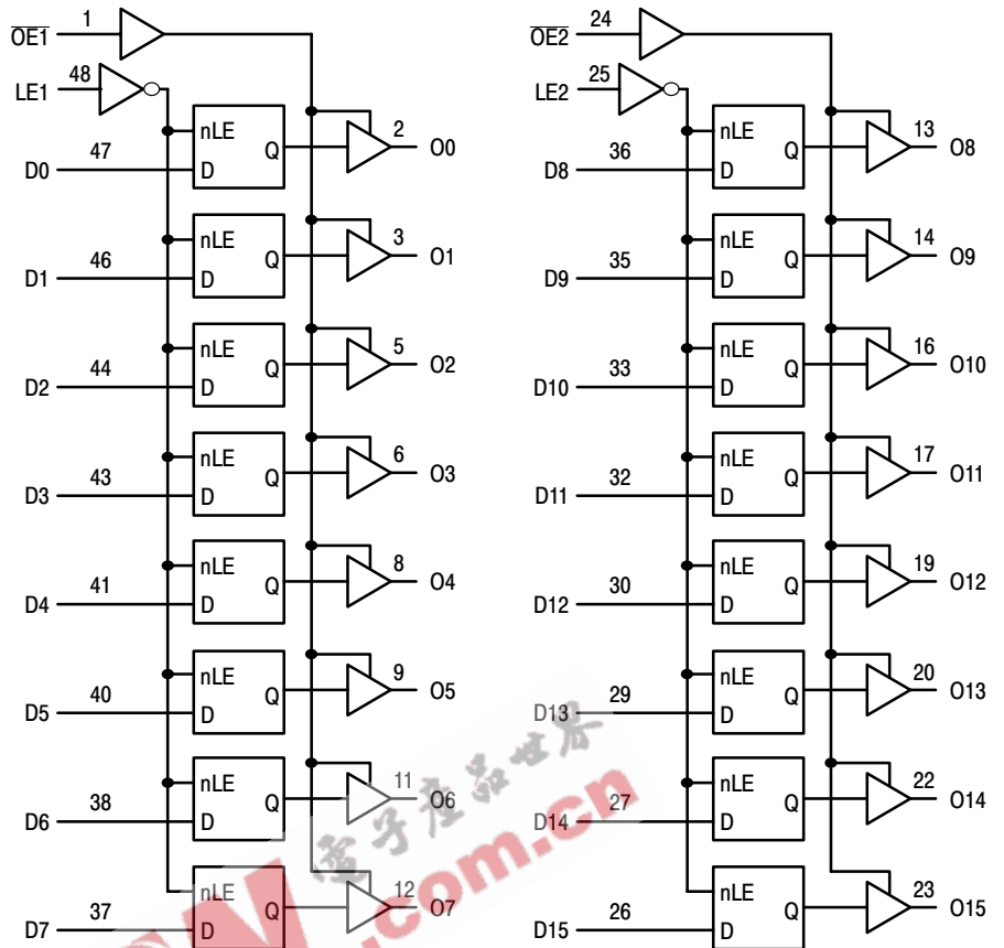
Figure 2. Logic Diagram
