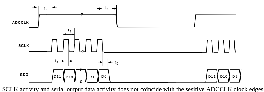
Figure 1. ADC Timing (ADCCLK \leq 1160 \text{ kHz} )
