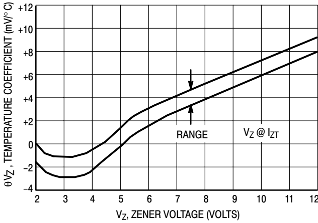
Figure 2. Temperature Coefficients
