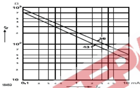
FIG.3- DYNAMIC RESISTANCE VS ZENER CURRENT
