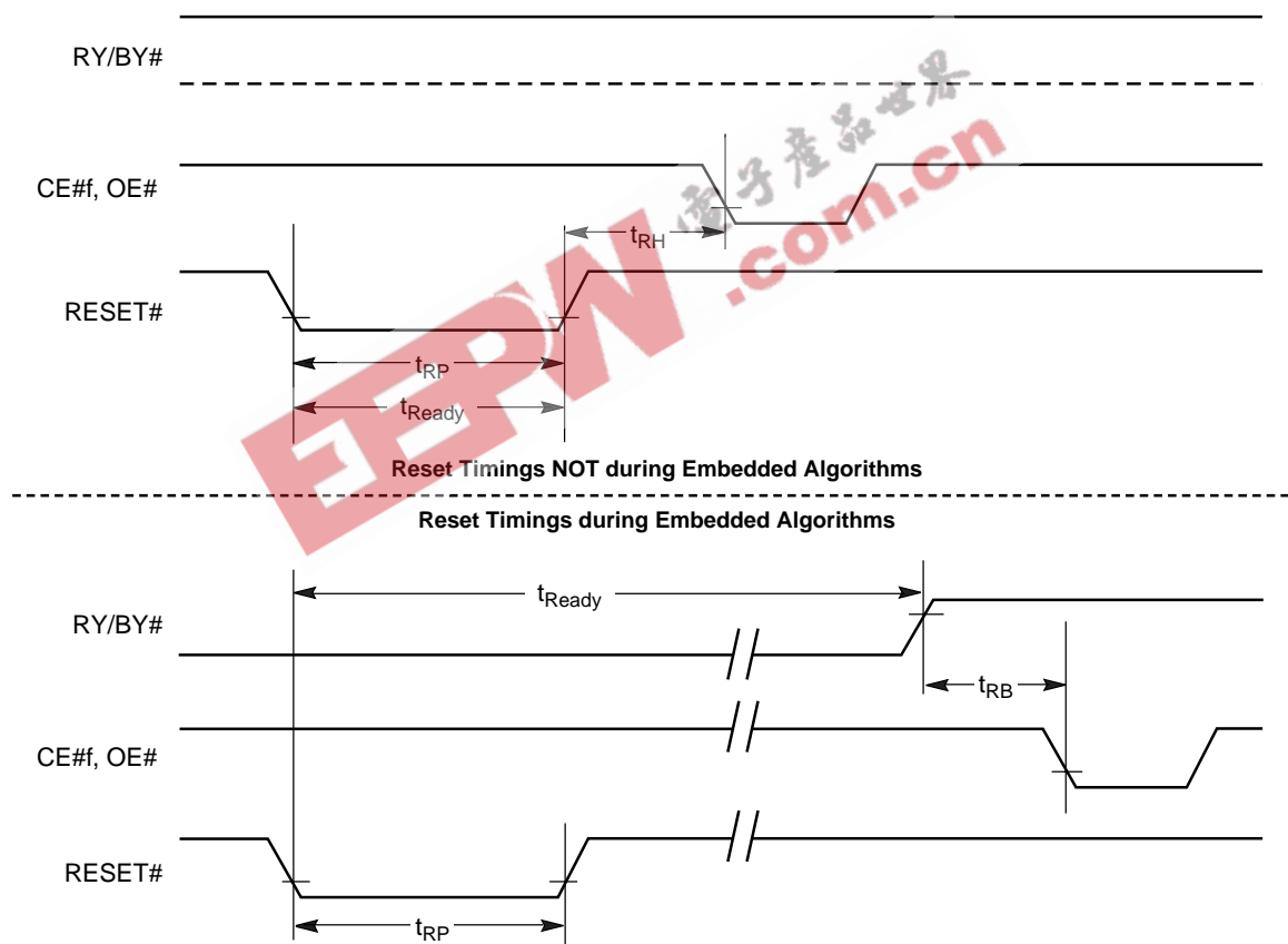
Figure 17. Reset Timings
