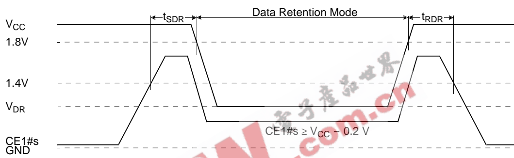
Figure 33. CE1#s Controlled Data Retention Mode
