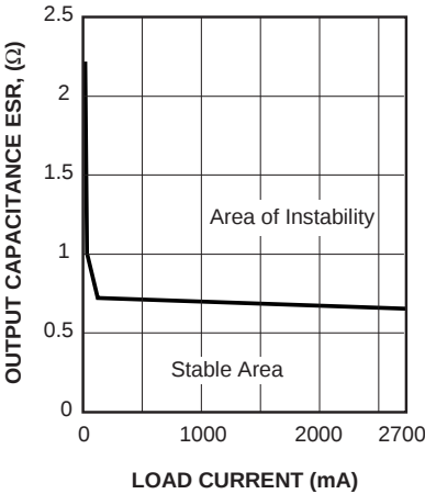
Figure 9. Stability Region
