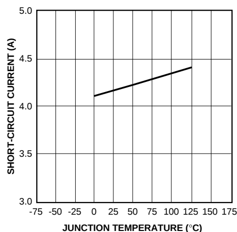
Figure 5. Short-Circuit Current vs. Temperature
