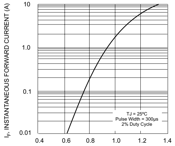
V_F , INSTANTANEOUS FORWARD VOLTAGE (VOLTS) Fig. 2 Typical Forward Characteristics
