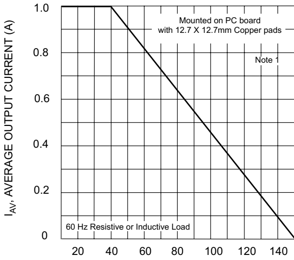
T_A , AMBIENT TEMPERATURE ( ^{\circ}C ) Fig. 1 Maximum Output Rectified Current
