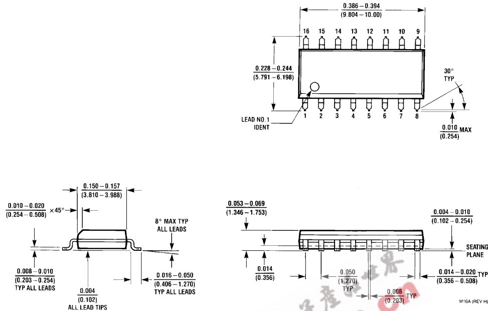
16-Lead Small Outline Molded Package (M) Order Number DM74LS157M or DM74LS158M NS Package Number M16A
