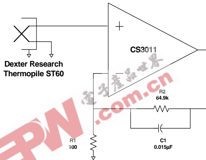
Figure 18. Thermopile Amplifier with a Gain of 650 V/V
