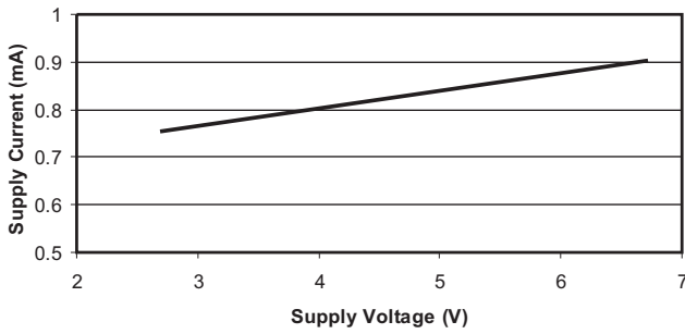
Figure 7. Supply Current vs. Voltage, 3011
