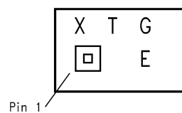
8 bump micro SMD Marking
