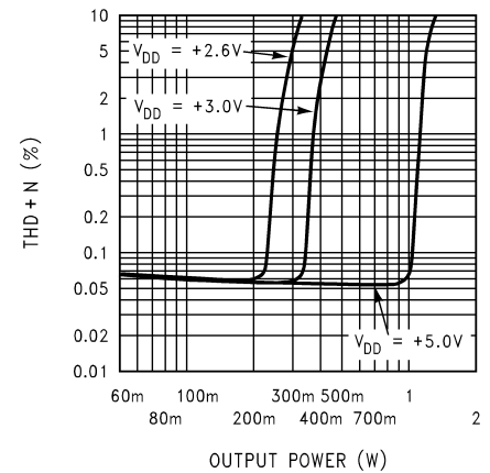
THD+N vs Power Out
