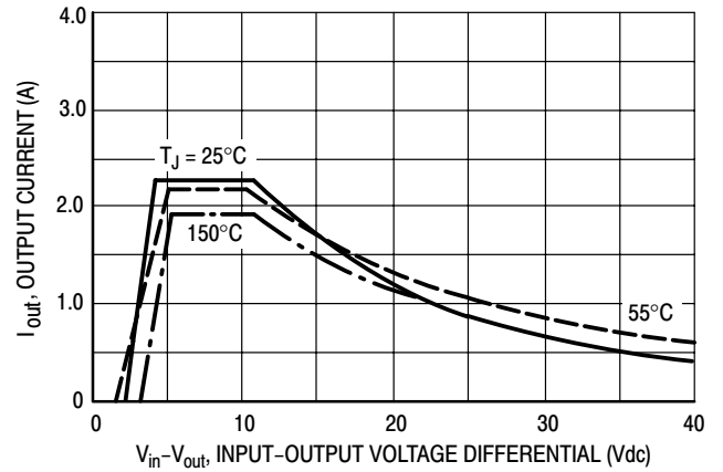
Figure 6. Current Limit
