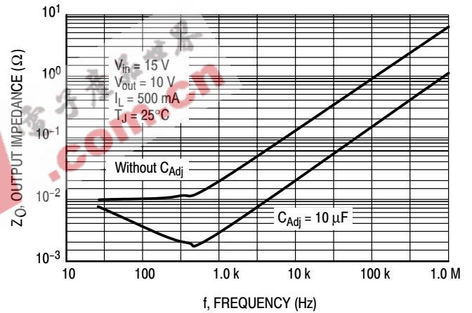
Figure 14. Output Impedance
