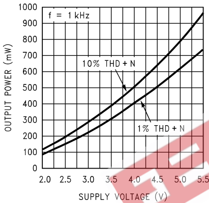
Output Power vs Supply Voltage, 16Ω
