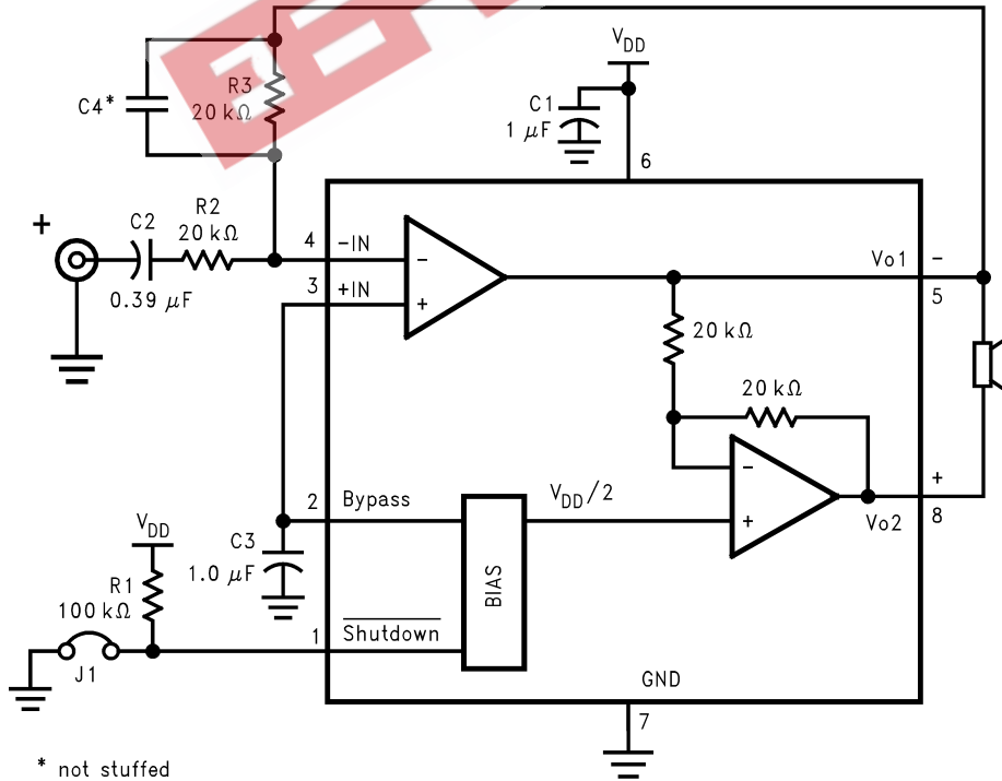
REFERENCE DESIGN BOARD SCHEMATIC
