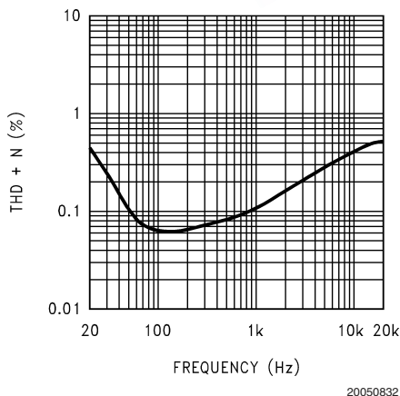
THD+N vs Frequency at V_{DD} = 2.6V , 8\Omega R_L , and PWR = 150mW
