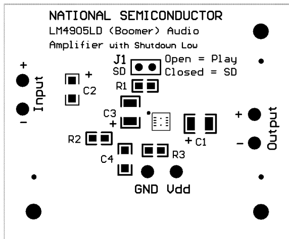
Silk Screen
