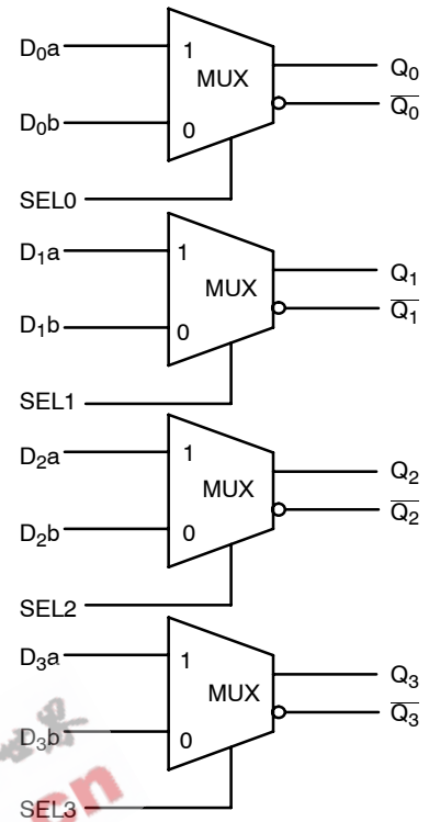
Figure 2. Logic Diagram
