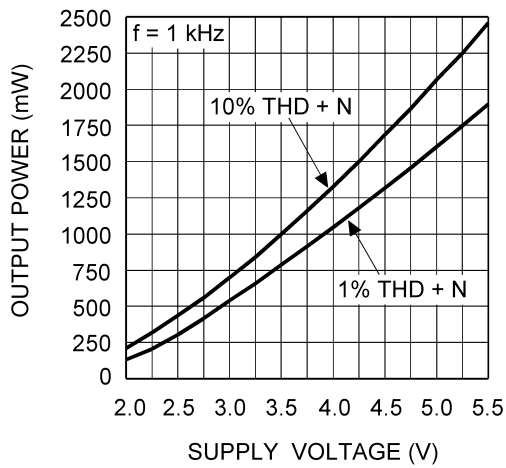
Output Power vs. Supply Voltage, 4Ω
