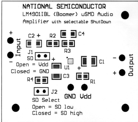
Silk Screen
