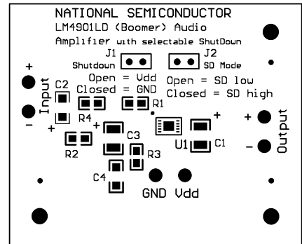
Silk Screen
