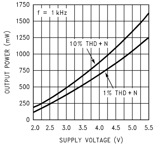
Output Power vs. Supply Voltage, 8Ω
