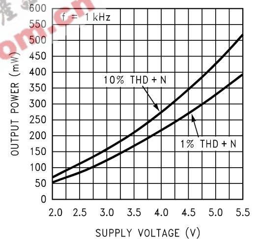
Output Power vs. Supply Voltage, 32Ω
