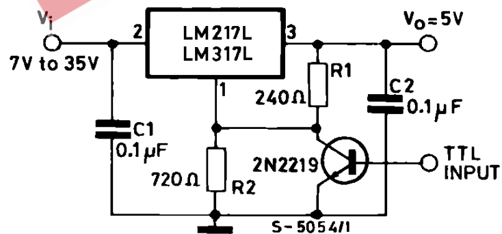
Figure 10: 5V Electronic Shut-down Regulator
