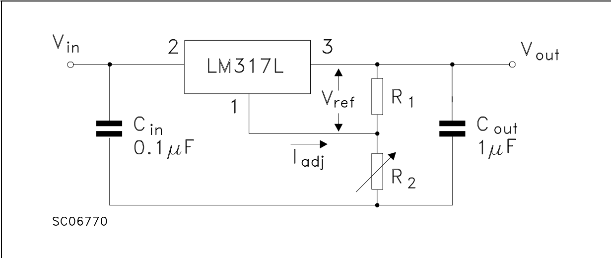
Figure 3: Test Circuit
