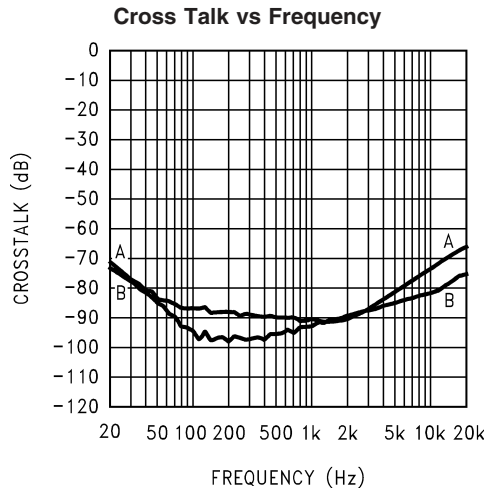
200428D1 V_{DD} = 5V, R_L = 8\Omega, A_V = 15.6dB, A = Left channel driven, right channel measured; B = Right channel driven, left channel measured
