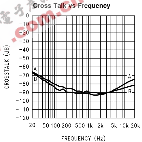
200428D4 V_{DD} = 3V, R_L = 8\Omega, A_V = 10dB, A = Left channel driven, right channel measured; B = Right channel driven, left channel measured
