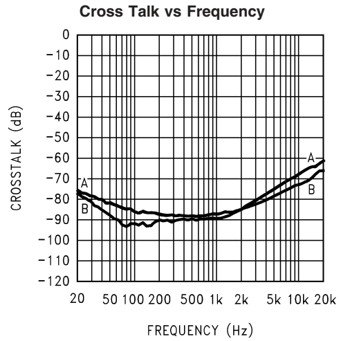
200428D2 V_{DD} = 5V, R_L = 8\Omega, A_V = 21.6dB, A = Left channel driven, right channel measured; B = Right channel driven, left channel measured
