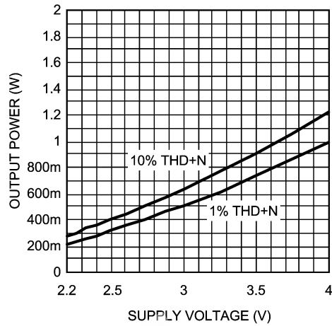
Output Power vs Supply Voltage R_L = 4\Omega
