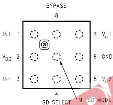
9 Bump micro SMD Package
