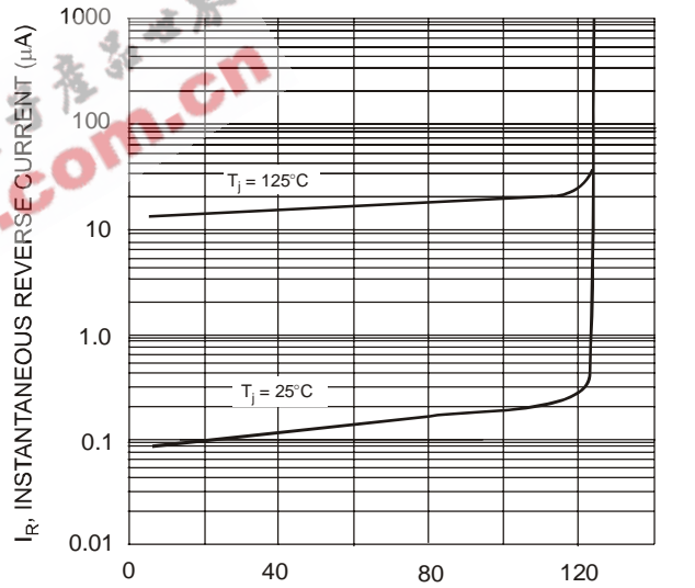
T_J = 125^\circ\text{C} T_J = 25^\circ\text{C} Fig. 4 Typical Reverse Characteristics
