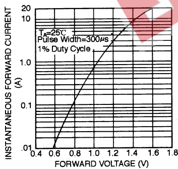
FIG.3-TYPICAL FORWARD CHARACTERISTICS
