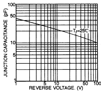
FIG.4-TYPICAL JUNCTION CAPACITANCE
