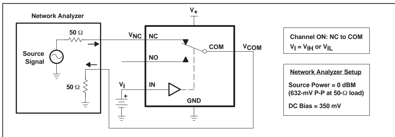
Figure 17. Bandwidth (BW)
