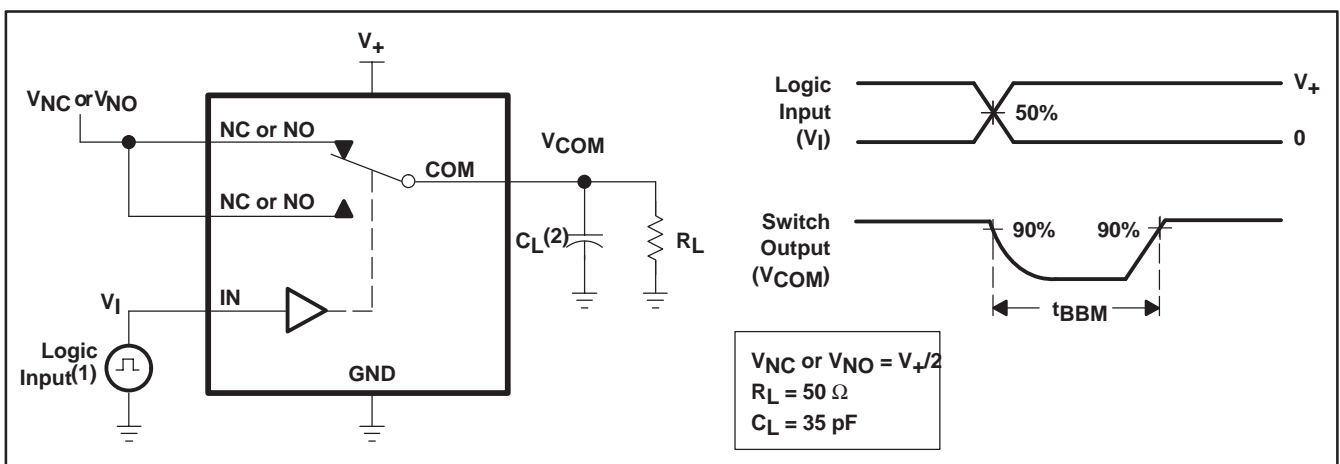
Figure 15. Turn-On (t ON ) and Turn-Off Time (t OFF )
