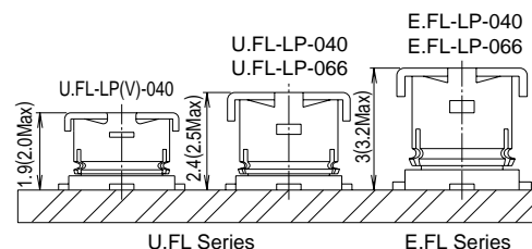
Mated Height Comparison (With Hirose Product)
