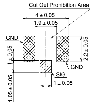
Recommended PCB Footprints
