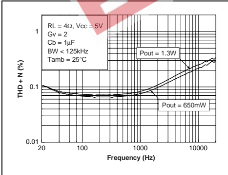
Figure 45: THD + N vs Frequency
