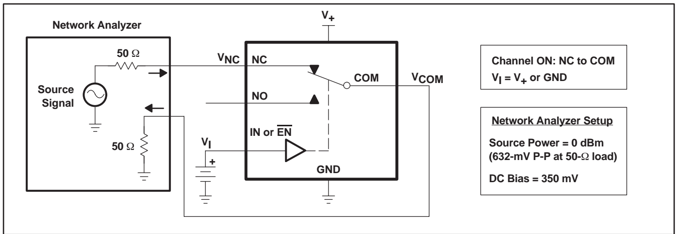
Figure 19. Bandwidth (BW)
