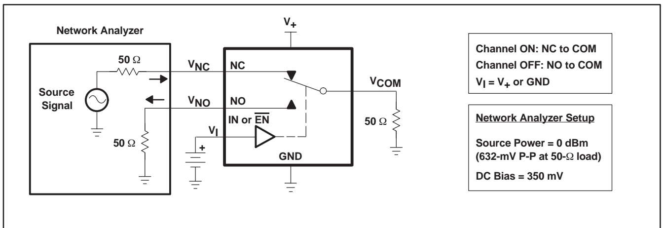
Figure 21. Crosstalk ( X_{TALK} )
