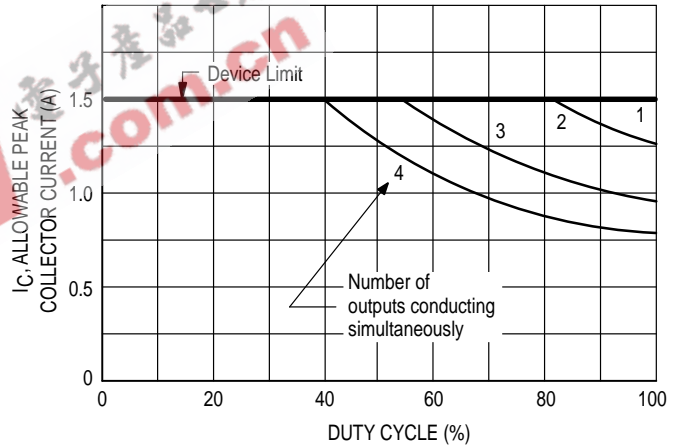
Figure 16. T_A = 50^\circ\text{C} w/Staver V-7 Heat Sink (27.5°C/W)
