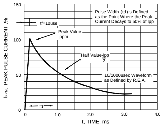
FIG.3- PULSE WAVEFORM
