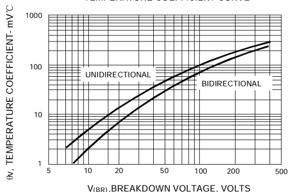
FIG.12- BREAKDOWN VOLTAGE TEMPERATURE COEFFICIENT CURVE
