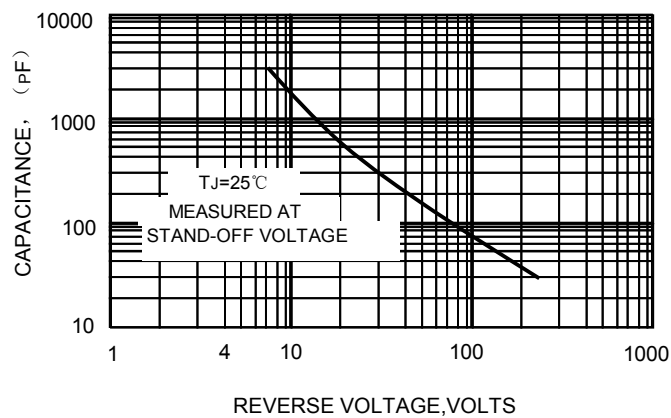
FIG.2-TYPICAL JUNCTION CAPACITANCE
