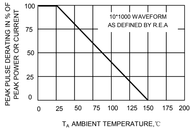
FIG.1-PULSE DERATING CURVE
