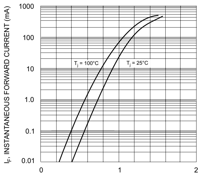
Fig. 1 Forward Characteristics 1N914, 1N914A
