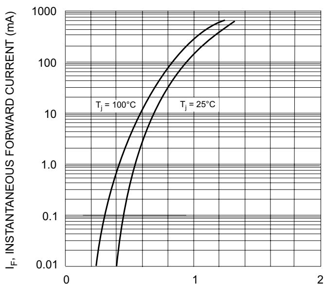
Fig. 2 Forward Characteristics 1N914B
