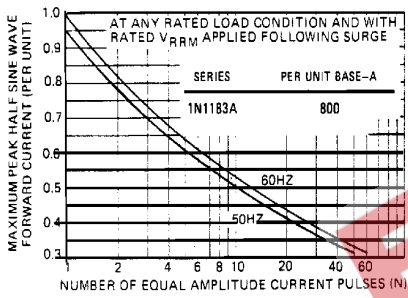
Fig. 10 - Maximum Non-Repetitive Surge Current Vs. Number of Current Pulses, 1N1183A Series
