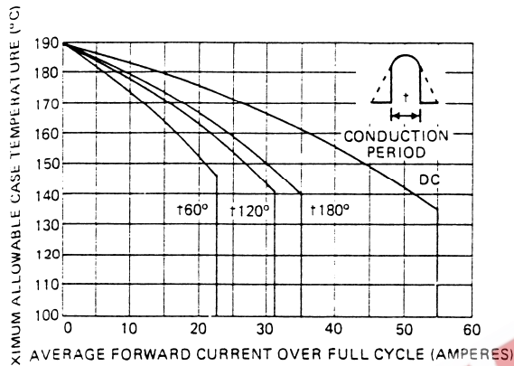
Fig. 1 - Maximum Allowable Case Temperature Vs. Average Forward Current, 1N1183 and 1N3765 Series
