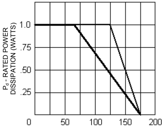
T_L - Lead Temperature ( ^{\circ}\text{C} ) 3/8" from body or T_A on FR4 PC Board FIGURE 1 Power Derating Curve
