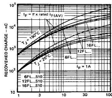
Fig. 19B — Maximum Recovered Charge Vs. Rate of Fall of Forward Current, All Series ___S10
