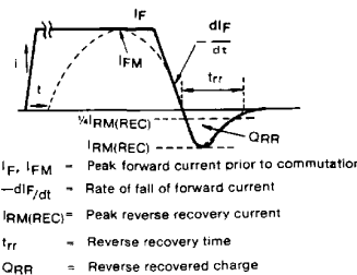
Fig. 4 - Reverse Recovery Time Test Waveform
