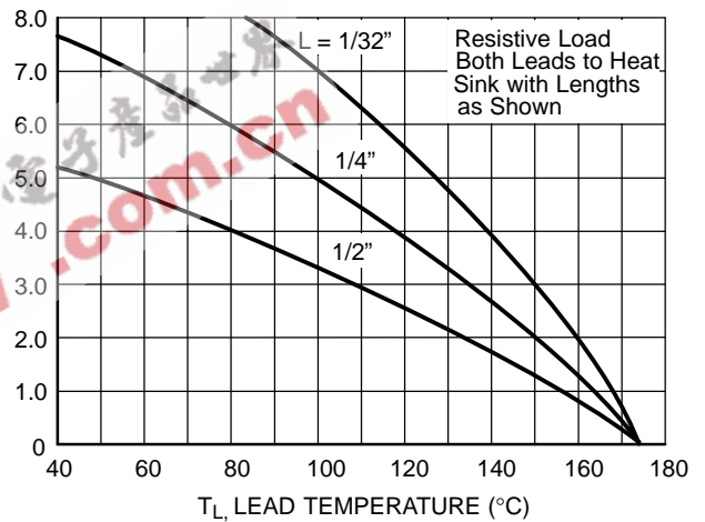
Figure 3. Current Derating Various Lead Lengths
