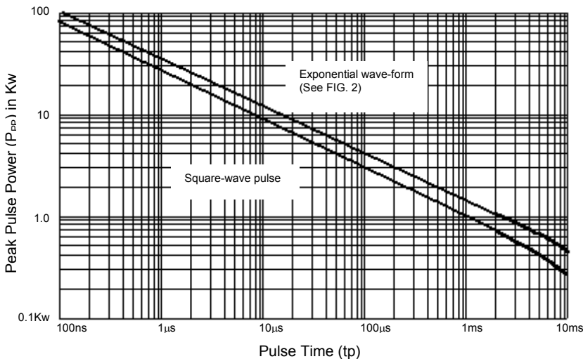
FIG. 1 - Non-repetitive peak pulse power rating curve
