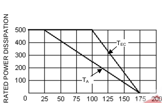
T_{EC} – End Cap Temperature ( ^\circ\text{C} ), or T_A Ambient Temperature on FR4 PC BOARD FIGURE 1 POWER DERATING CURVE
