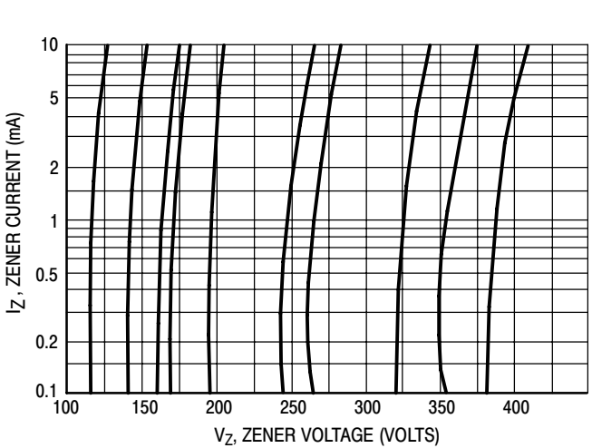
Figure 9. V_Z = 100 thru 400 Volts
