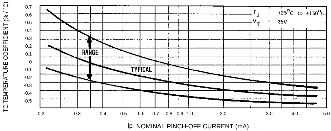
FIGURE 2 TEMPERATURE COEFFICIENT
