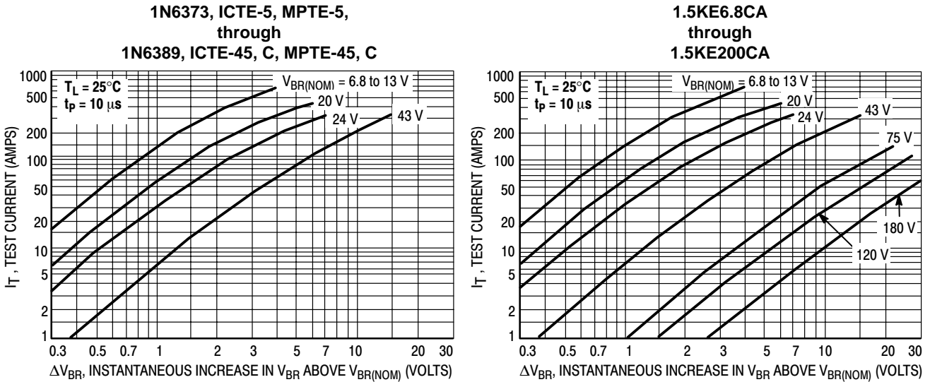
Figure 6. Dynamic Impedance
