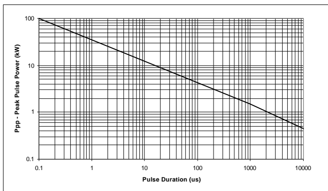
PEAK PULSE POWER vs. PULSE TIME
