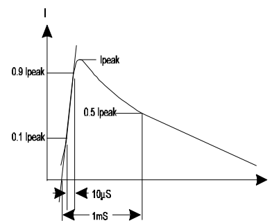
10x1000µs IMPULSE WAVEFORM
