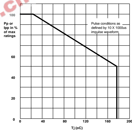
PULSE DERATING CURVE
