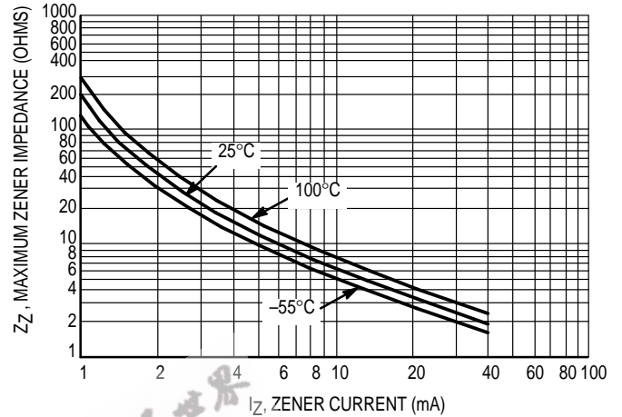
Figure 5. 1N821A Series
